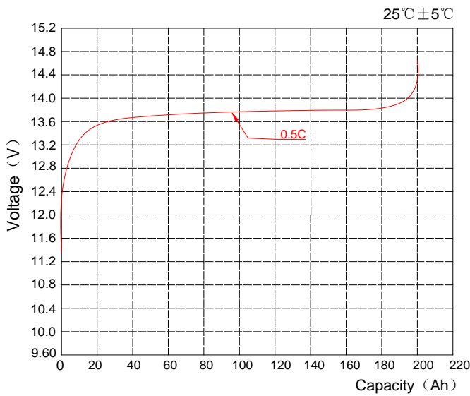
charge curve
