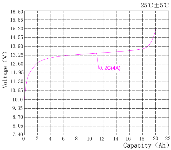
charge curve
