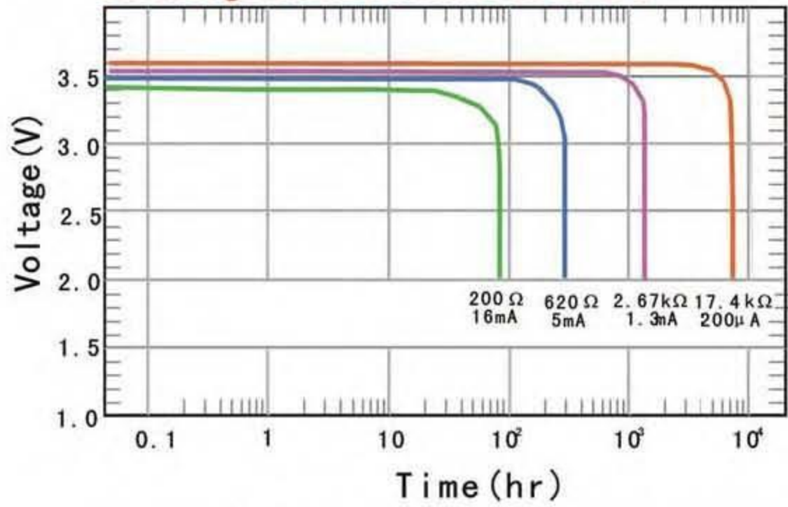
Capacity VS. Current
