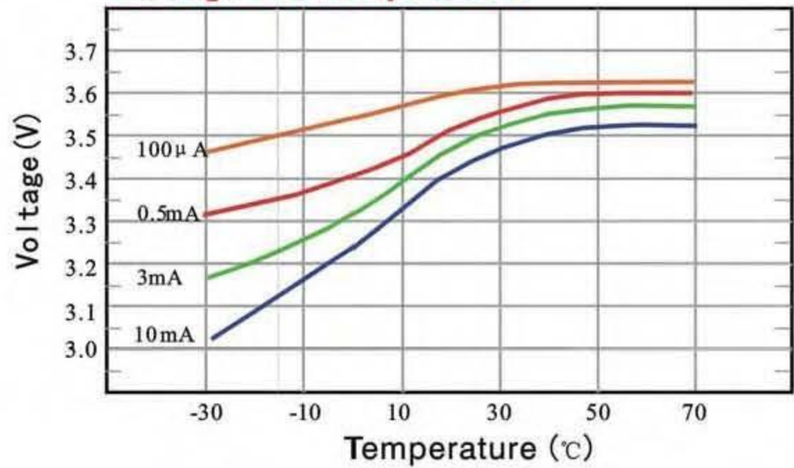
Voltage VS. Temperature
